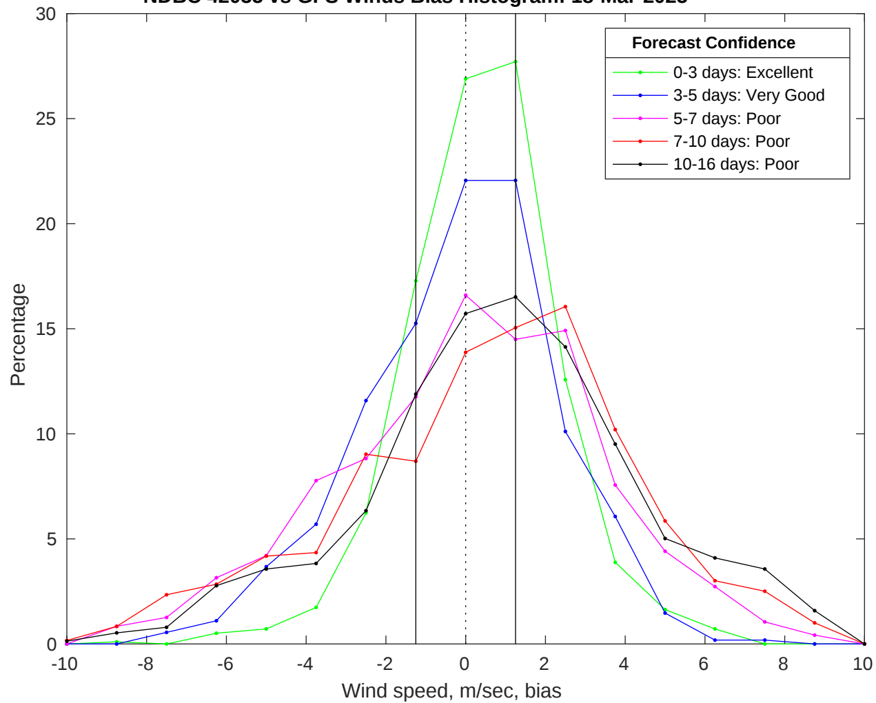
NDBC 42035 vs GFS Winds Bias Histogram: 18-Mar-2025
