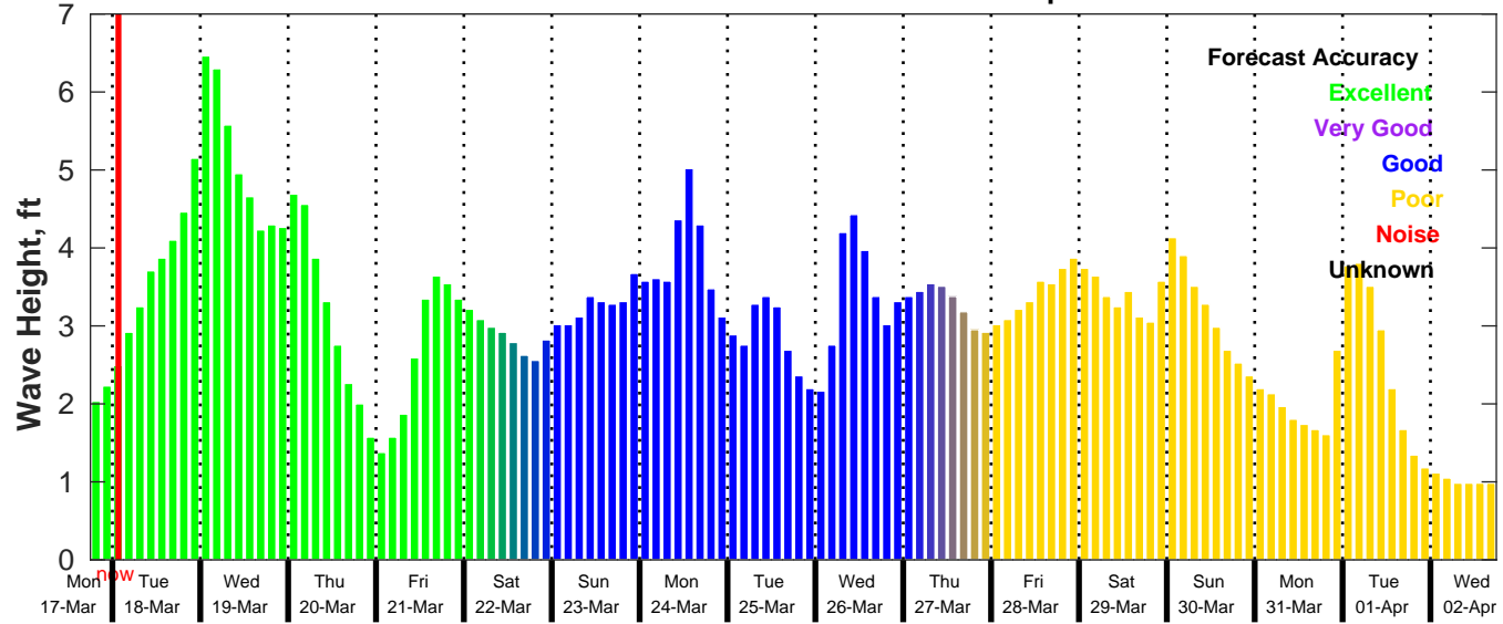
GFS Wave Forecast for NDBC 42035 from 17-Mar-2025 18:00:00 to 02-Apr-2025 18:00:00
