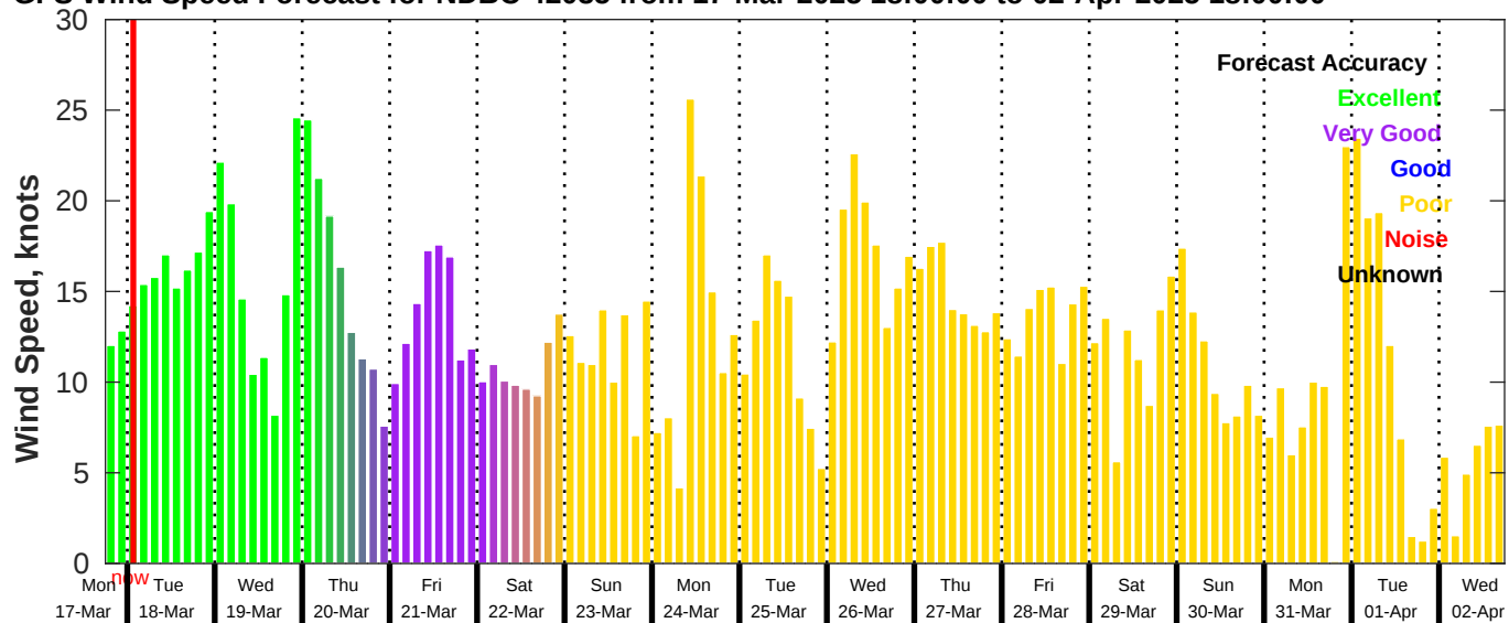
GFS Wind Speed Forecast for NDBC 42035 from 17-Mar-2025 18:00:00 to 02-Apr-2025 18:00:00
