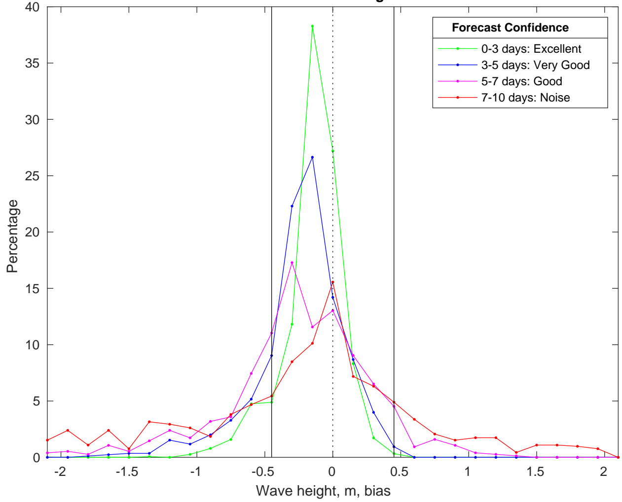
NDBC 42036 vs CMEMS Waves Bias Histogram: 18-Mar-2025
