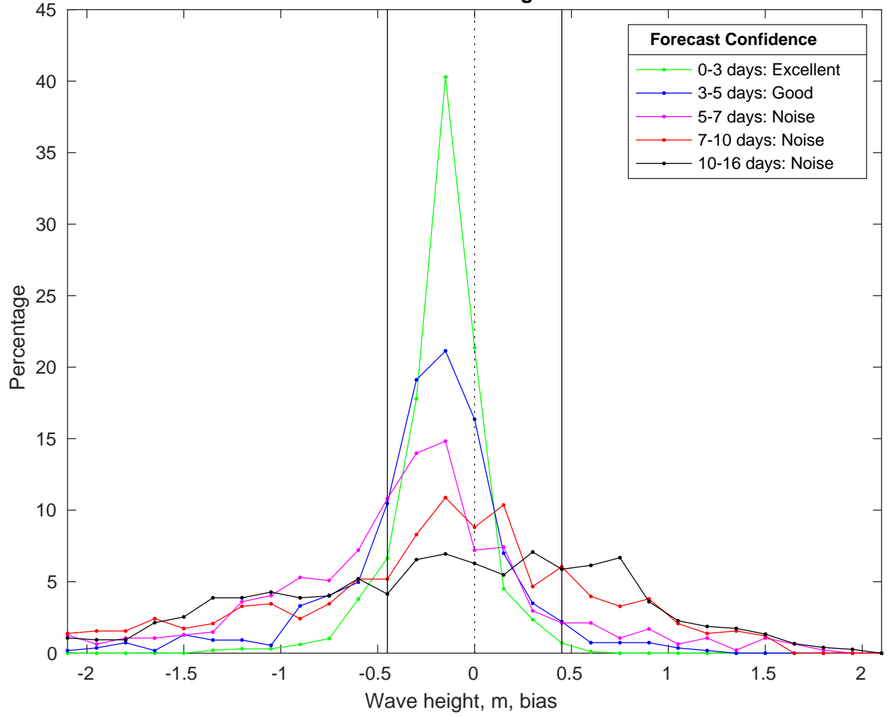
NDBC 42036 vs GFS Waves Bias Histogram: 18-Mar-2025
