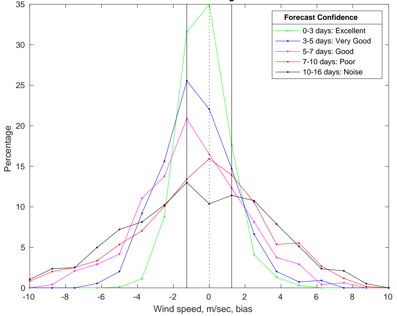
NDBC 42036 vs GFS Winds Bias Histogram: 18-Mar-2025
