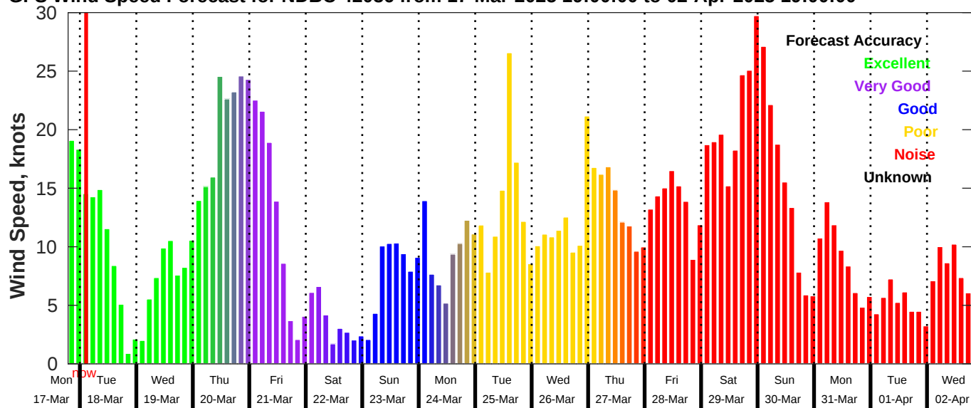
GFS Wind Speed Forecast for NDBC 42036 from 17-Mar-2025 19:00:00 to 02-Apr-2025 19:00:00
