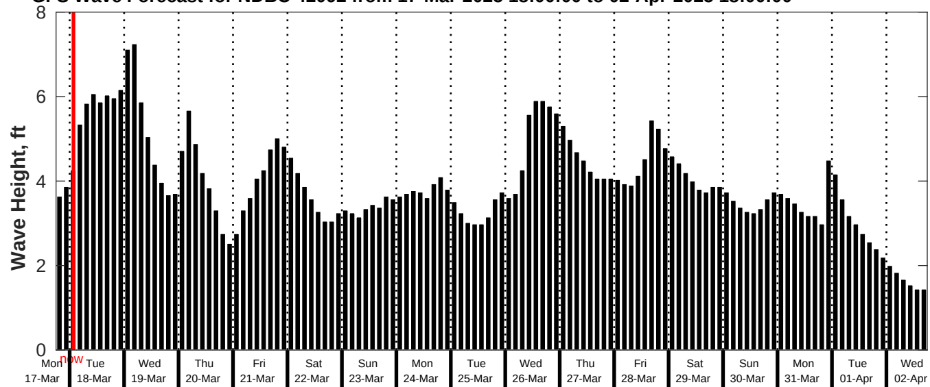
GFS Wave Forecast for NDBC 42092 from 17-Mar-2025 18:00:00 to 02-Apr-2025 18:00:00
