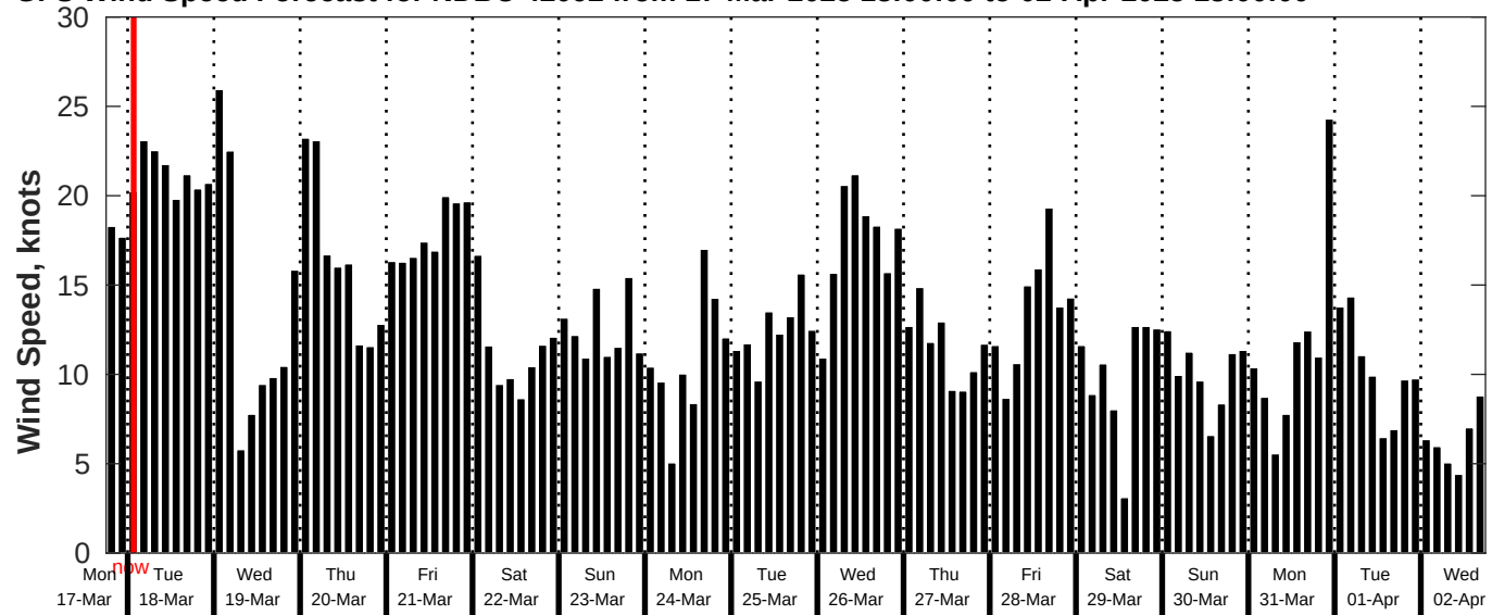
GFS Wind Speed Forecast for NDBC 42092 from 17-Mar-2025 18:00:00 to 02-Apr-2025 18:00:00
