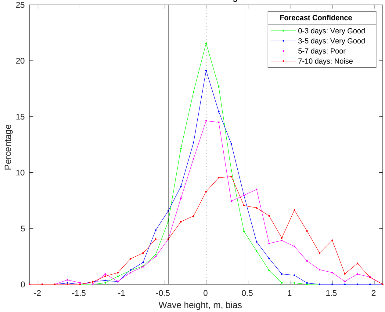
NDBC 46011 vs CMEMS Waves Bias Histogram: 18-Mar-2025
