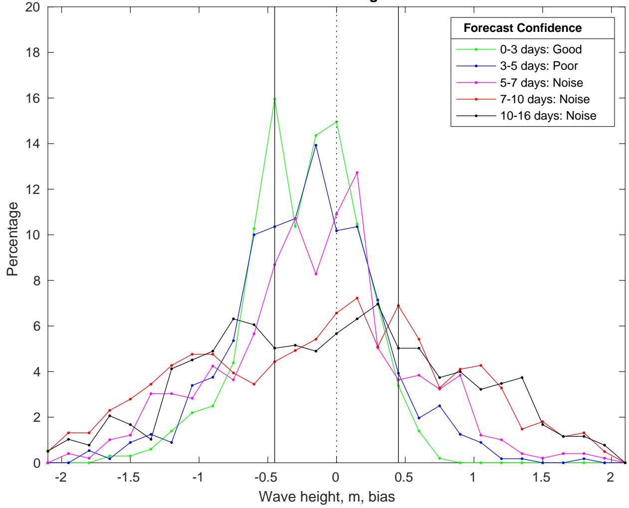
NDBC 46011 vs GFS Waves Bias Histogram: 18-Mar-2025
