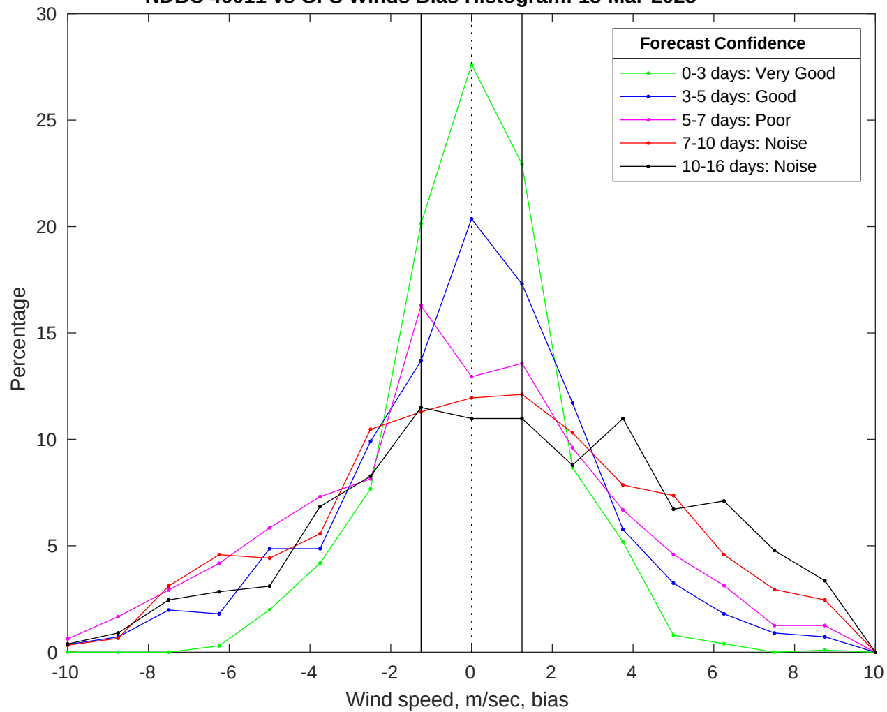
NDBC 46011 vs GFS Winds Bias Histogram: 18-Mar-2025
