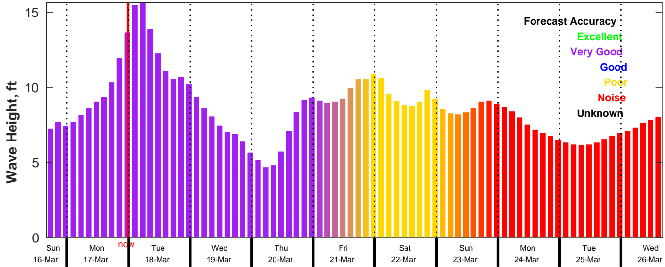
CMEMS Wave Forecast for NDBC 46011 from 16-Mar-2025 16:00:00 to 26-Mar-2025 16:00:00
