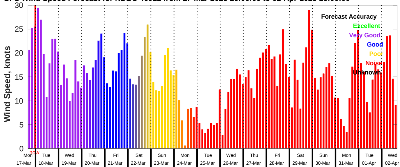
GFS Wind Speed Forecast for NDBC 46011 from 17-Mar-2025 16:00:00 to 02-Apr-2025 16:00:00
