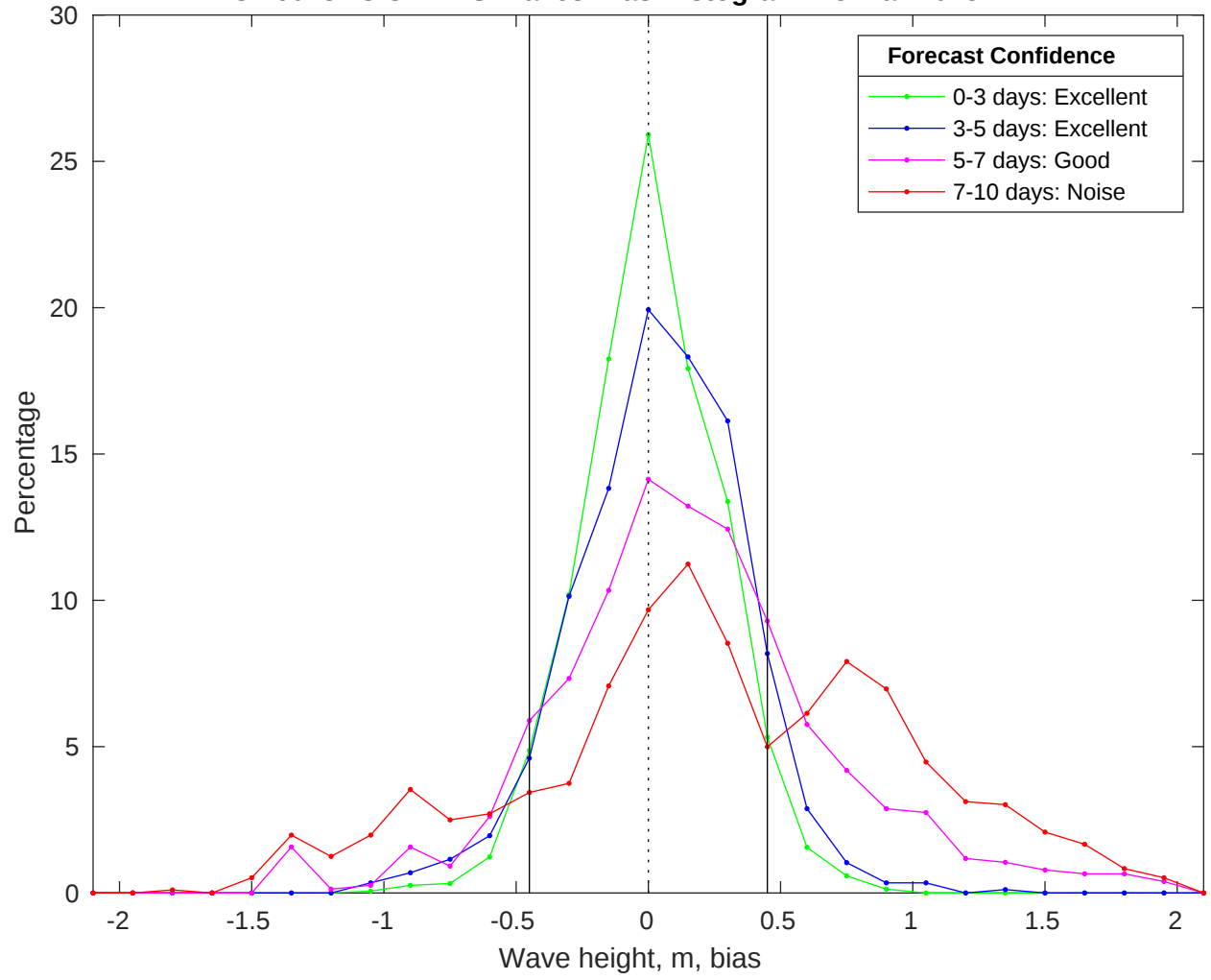
NDBC 46028 vs CMEMS Waves Bias Histogram: 18-Mar-2025
