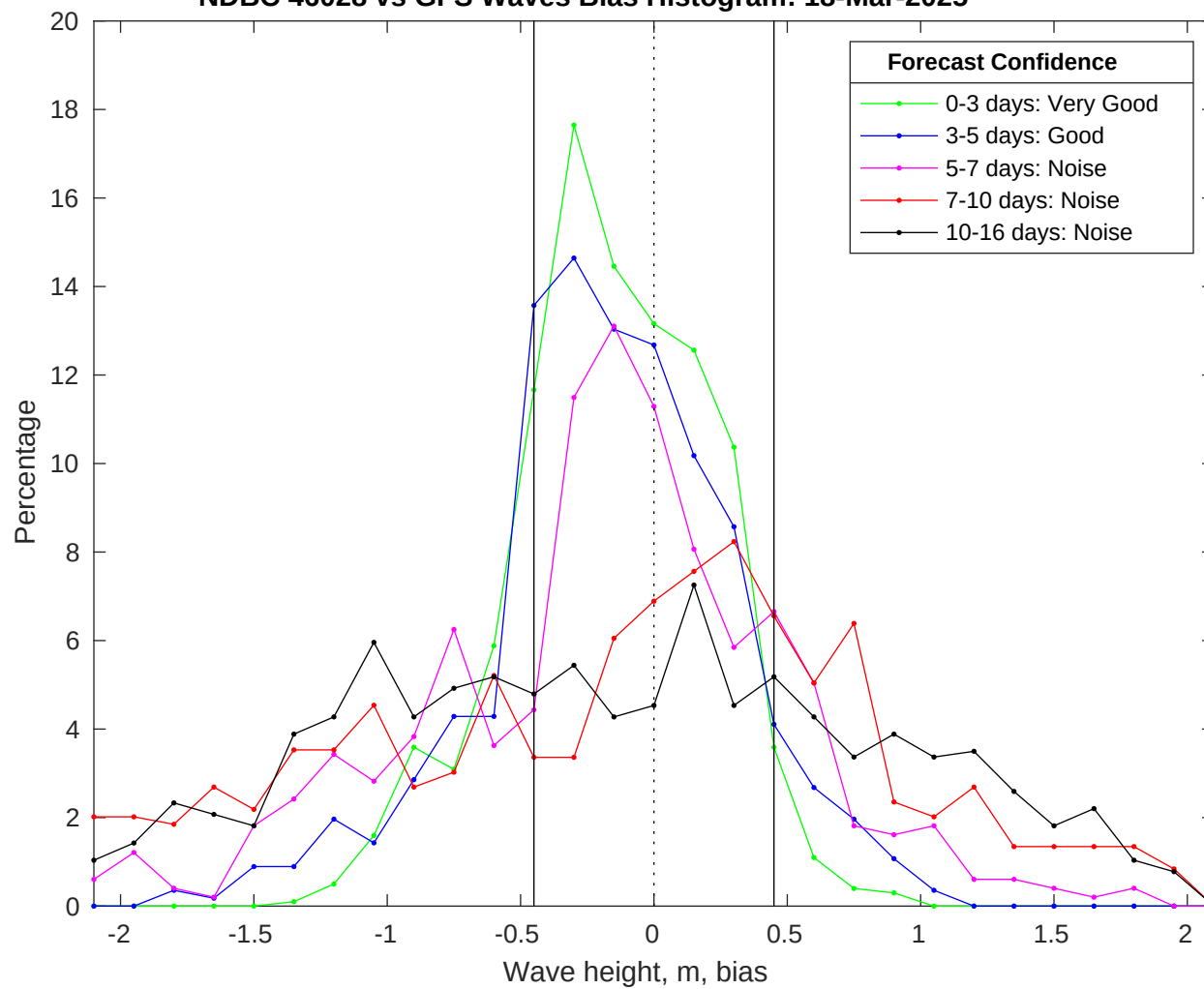
NDBC 46028 vs GFS Waves Bias Histogram: 18-Mar-2025
