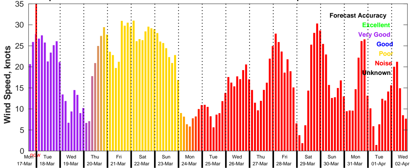
GFS Wind Speed Forecast for NDBC 46028 from 17-Mar-2025 16:00:00 to 02-Apr-2025 16:00:00
