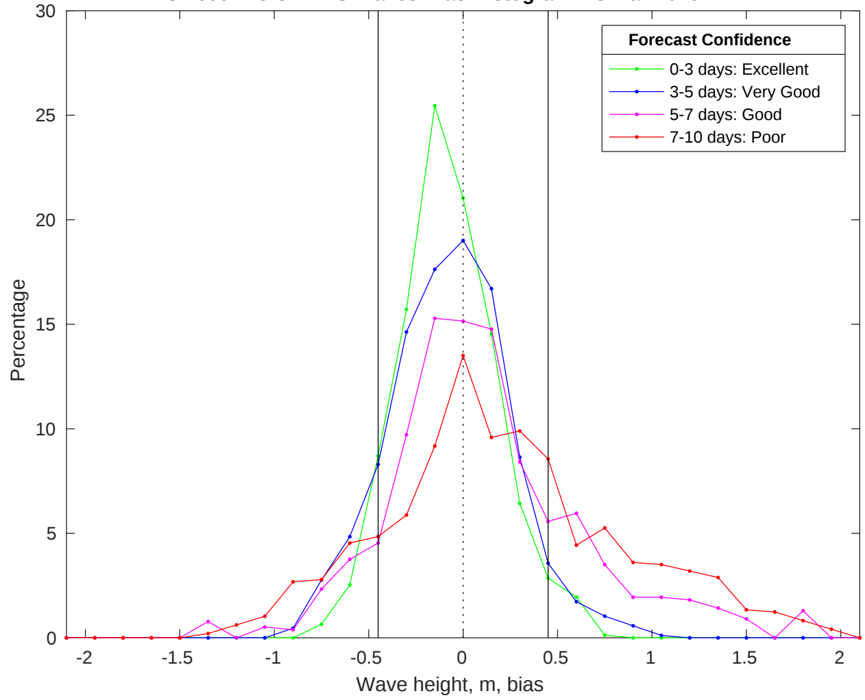
NDBC 46054 vs CMEMS Waves Bias Histogram: 18-Mar-2025
