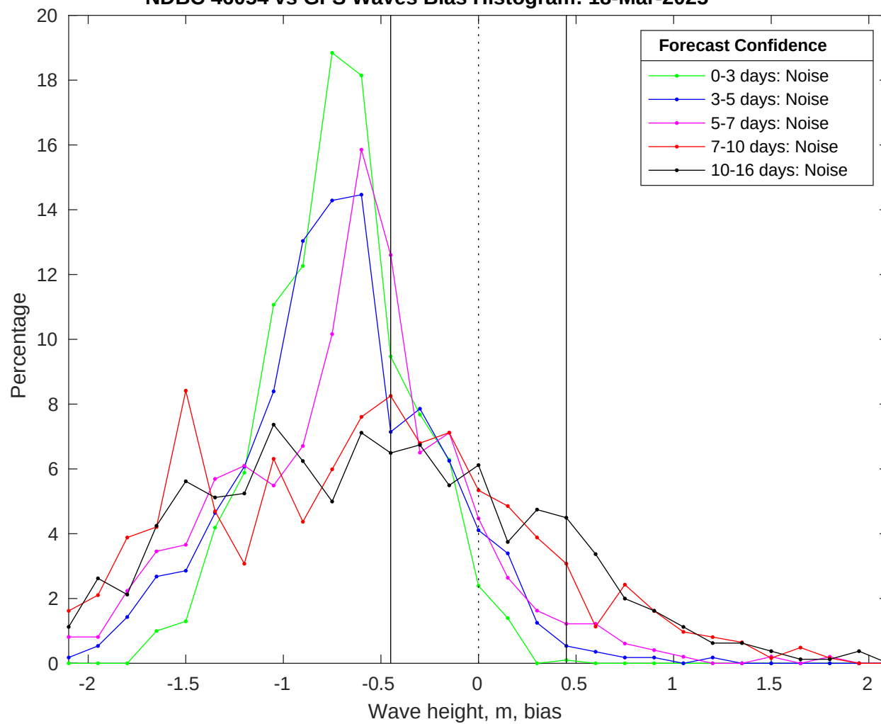
NDBC 46054 vs GFS Waves Bias Histogram: 18-Mar-2025
