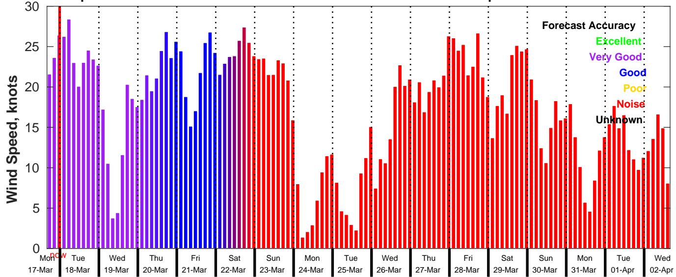
GFS Wind Speed Forecast for NDBC 46054 from 17-Mar-2025 16:00:00 to 02-Apr-2025 16:00:00
