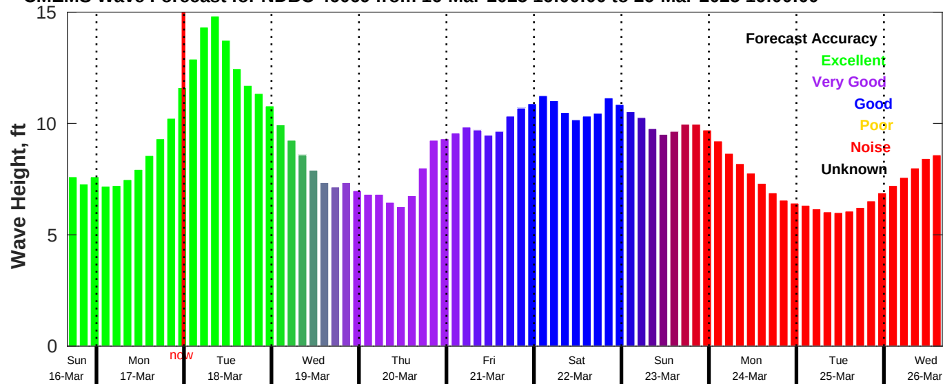
CMEMS Wave Forecast for NDBC 46069 from 16-Mar-2025 16:00:00 to 26-Mar-2025 16:00:00
