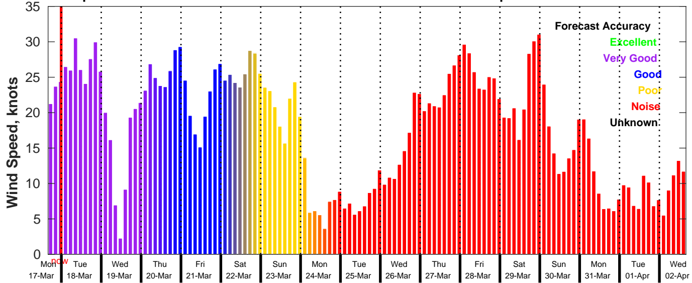
GFS Wind Speed Forecast for NDBC 46069 from 17-Mar-2025 16:00:00 to 02-Apr-2025 16:00:00
