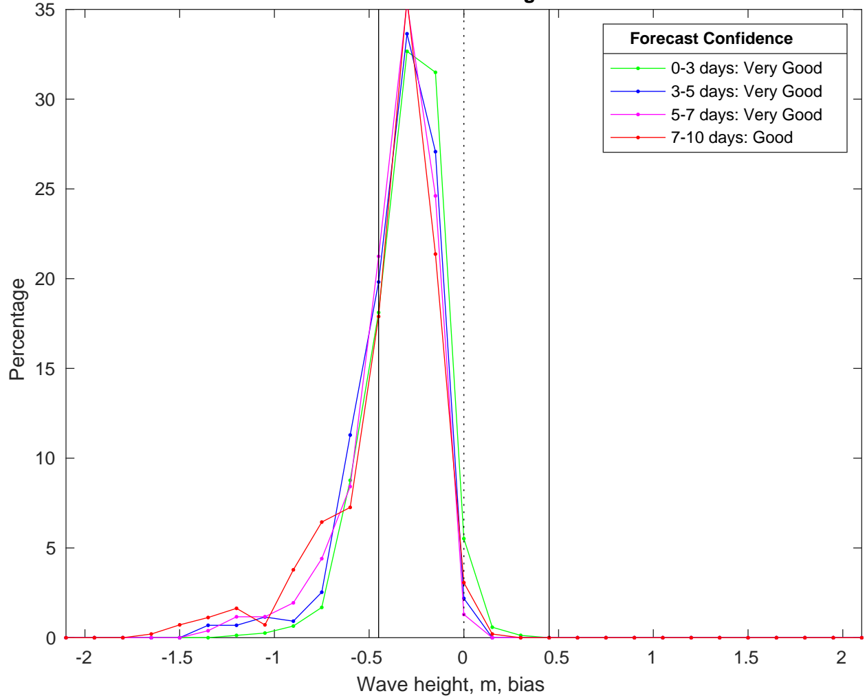
NDBC 51209 vs CMEMS Waves Bias Histogram: 18-Mar-2025
