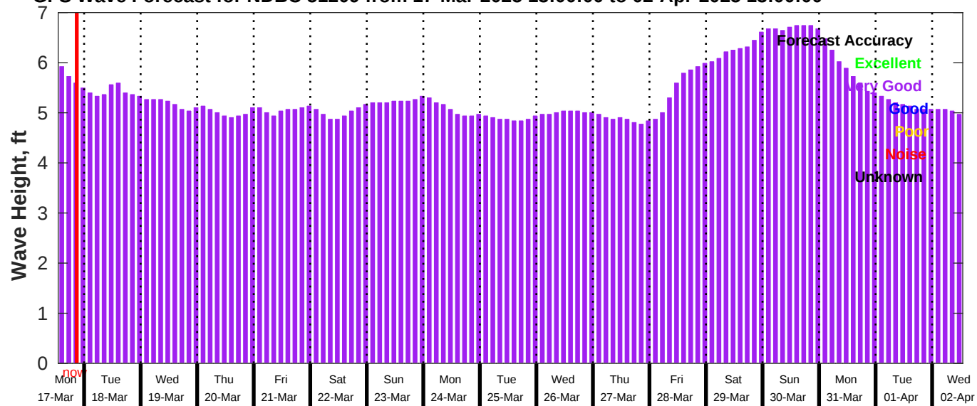
GFS Wave Forecast for NDBC 51209 from 17-Mar-2025 13:00:00 to 02-Apr-2025 13:00:00
