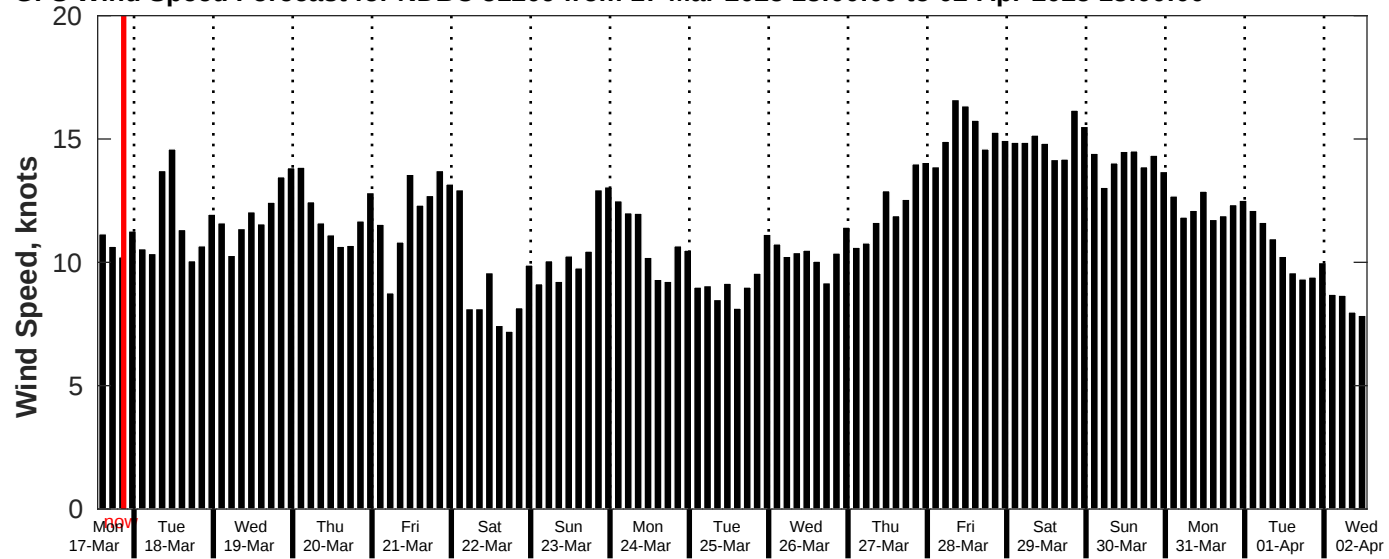
GFS Wind Speed Forecast for NDBC 51209 from 17-Mar-2025 13:00:00 to 02-Apr-2025 13:00:00
