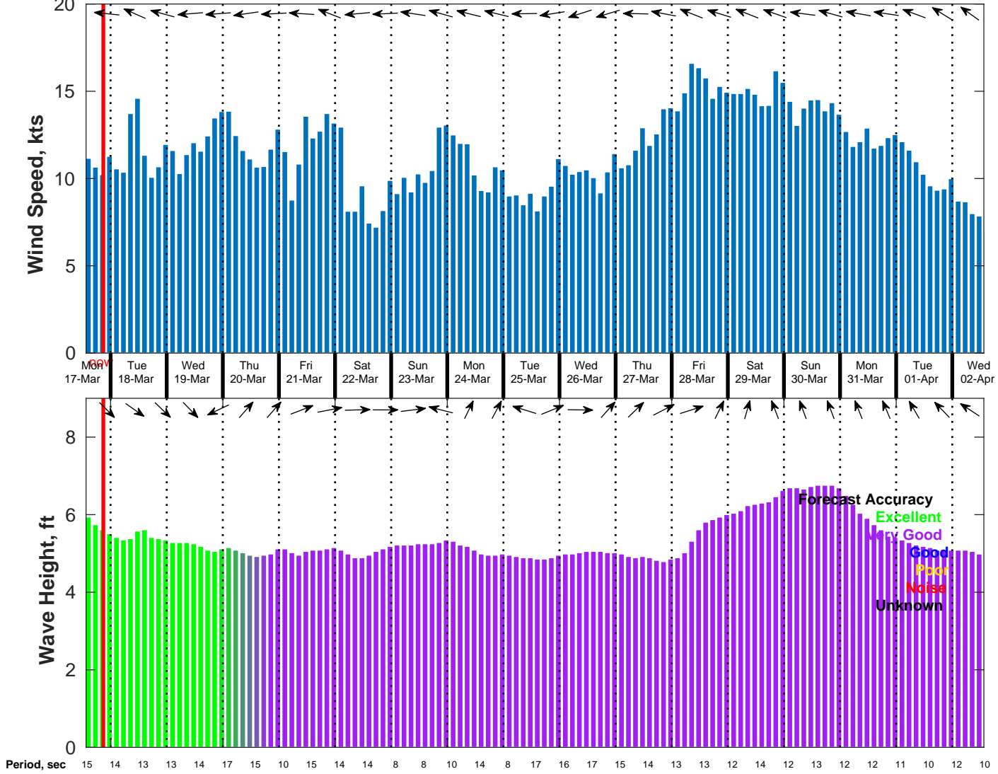
Wind & Wave Forecast for NDBC 51209 from 17-Mar-2025 13:00:00 to 02-Apr-2025 13:00:00
