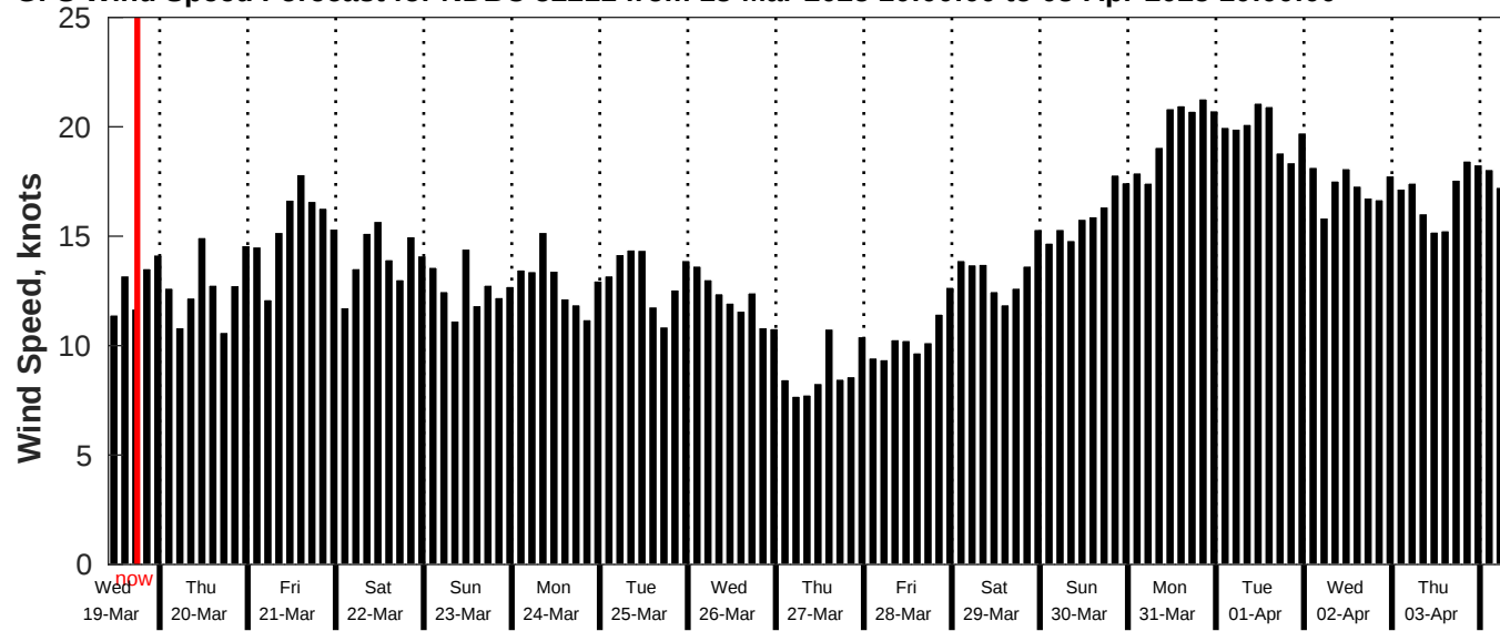
GFS Wind Speed Forecast for NDBC 52211 from 18-Mar-2025 10:00:00 to 03-Apr-2025 10:00:00
