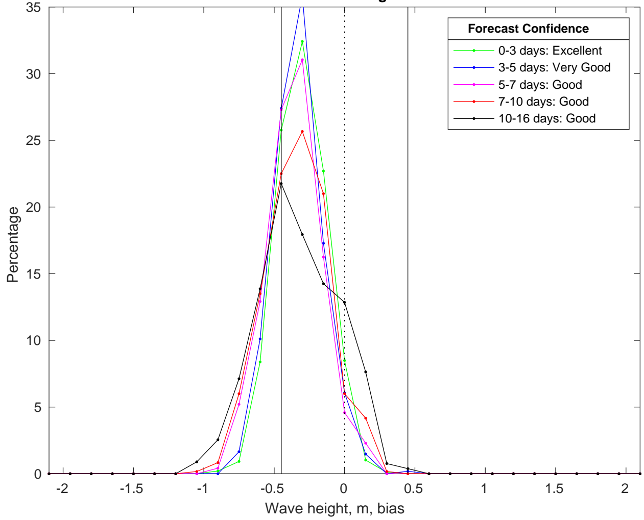
NDBC 52212 vs GFS Waves Bias Histogram: 18-Mar-2025
