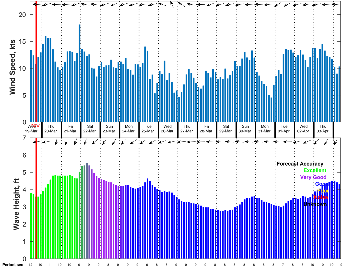
Wind & Wave Forecast for NDBC 52212 from 18-Mar-2025 09:00:00 to 03-Apr-2025 09:00:00
