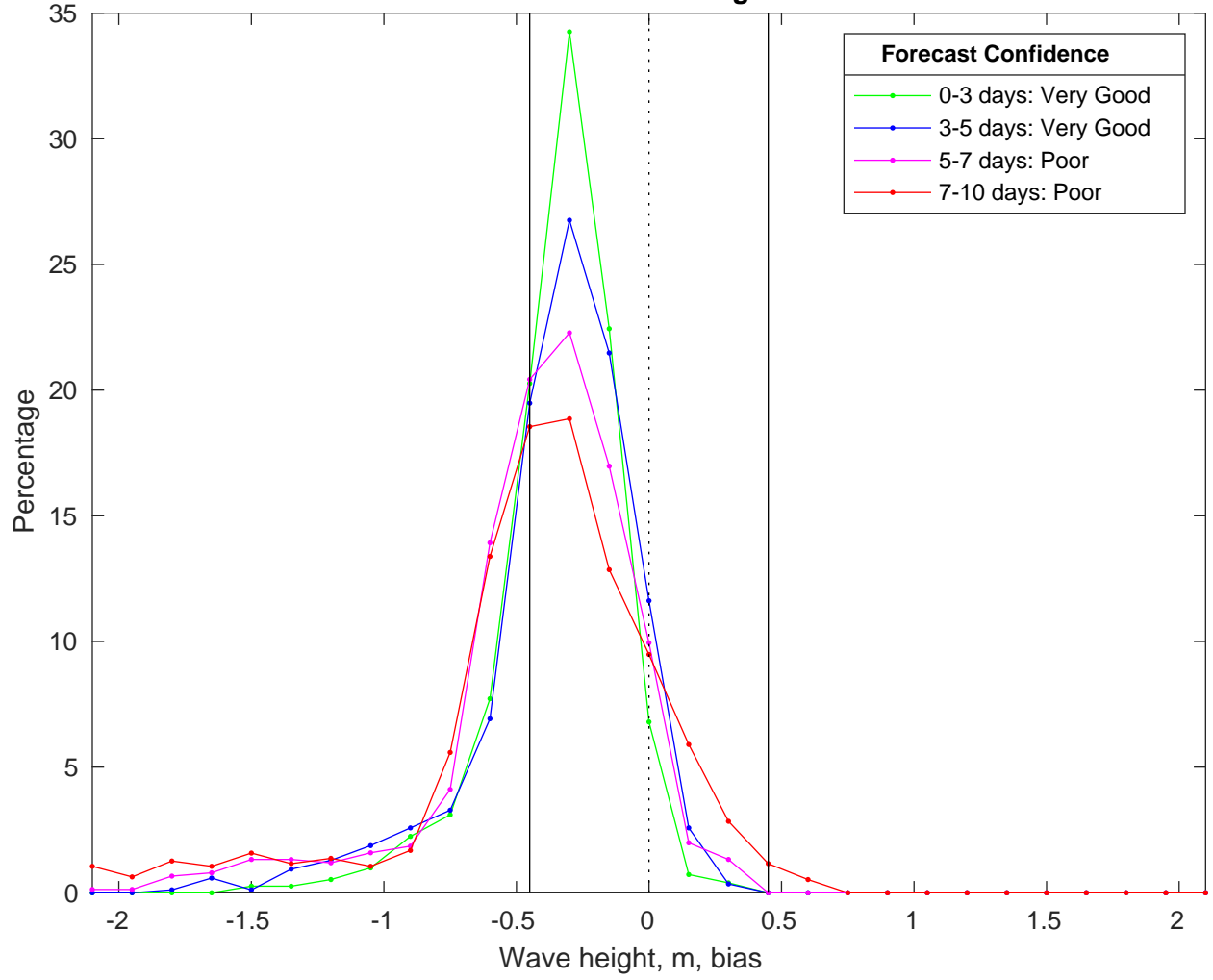
NDBC 52213 vs CMEMS Waves Bias Histogram: 18-Mar-2025
