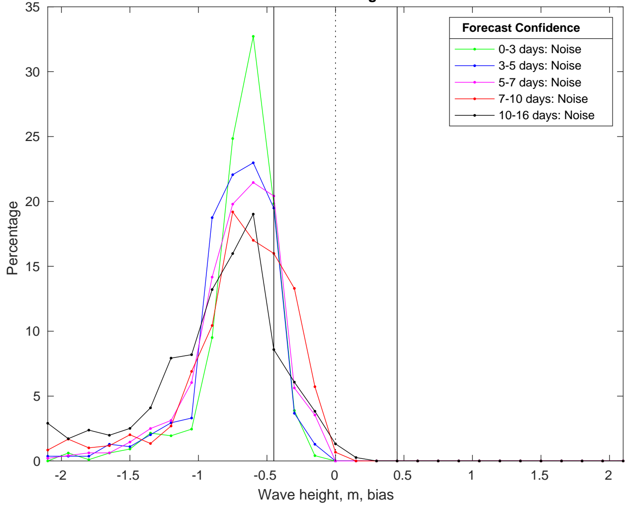
NDBC 52213 vs GFS Waves Bias Histogram: 18-Mar-2025
