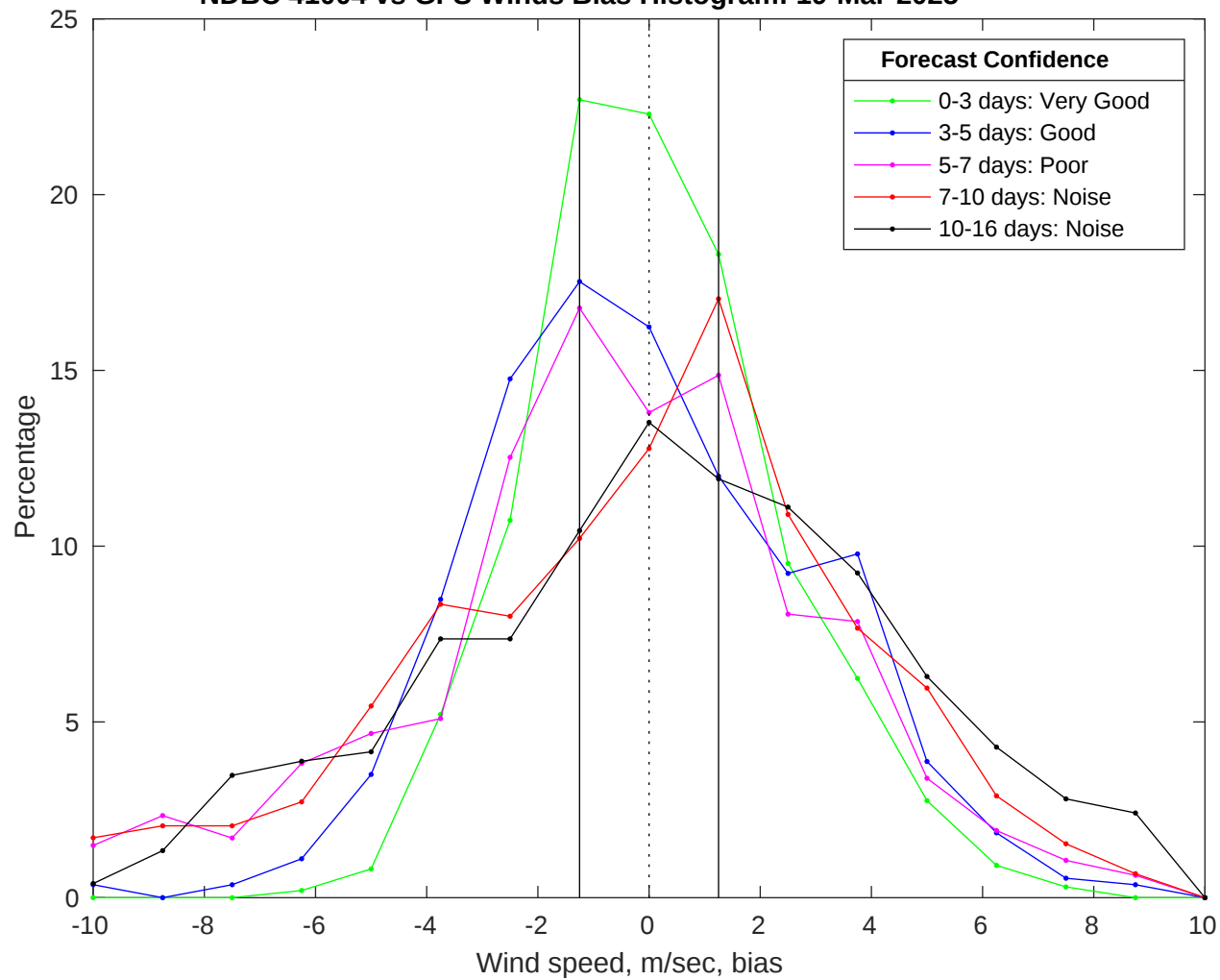
NDBC 41004 vs GFS Winds Bias Histogram: 19-Mar-2025
