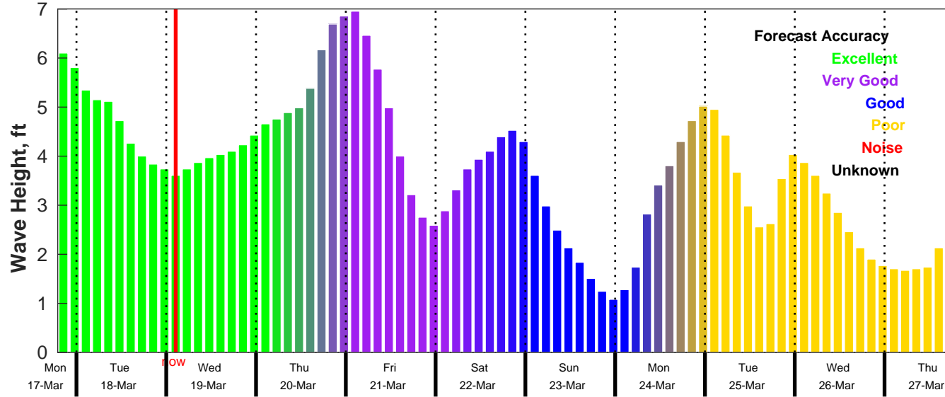
CMEMS Wave Forecast for NDBC 41004 from 17-Mar-2025 19:00:00 to 27-Mar-2025 19:00:00
