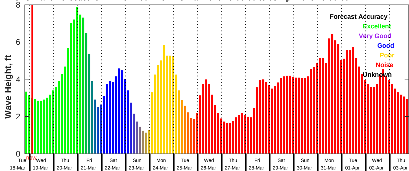
GFS Wave Forecast for NDBC 41004 from 18-Mar-2025 19:00:00 to 03-Apr-2025 19:00:00
