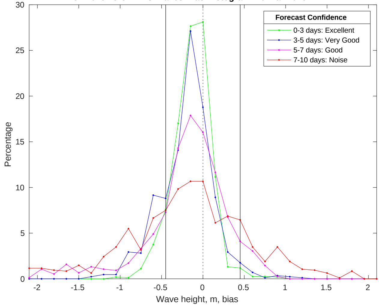
NDBC 41013 vs CMEMS Waves Bias Histogram: 19-Mar-2025
