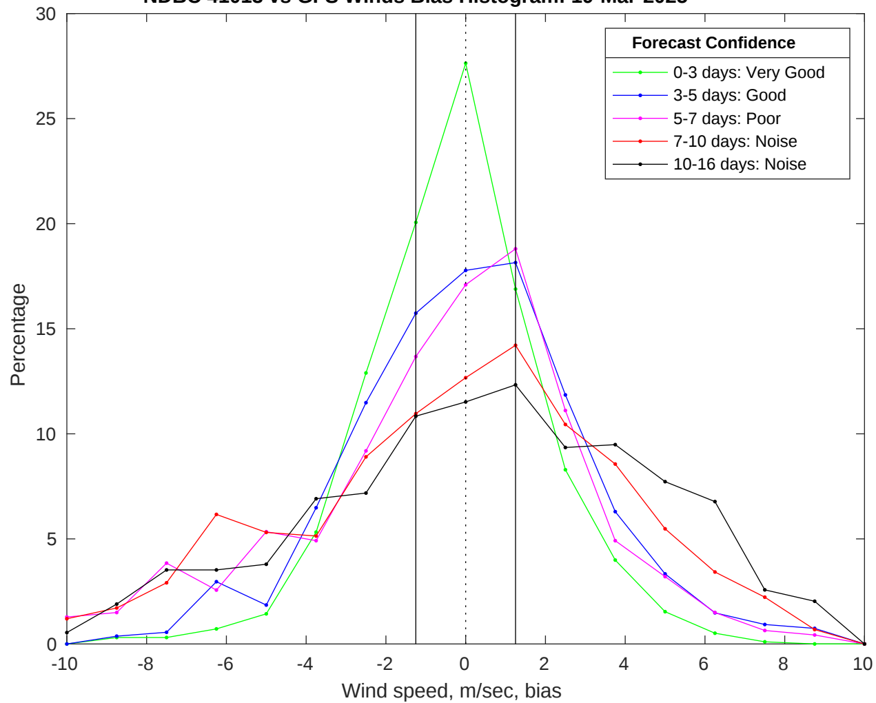
NDBC 41013 vs GFS Winds Bias Histogram: 19-Mar-2025
