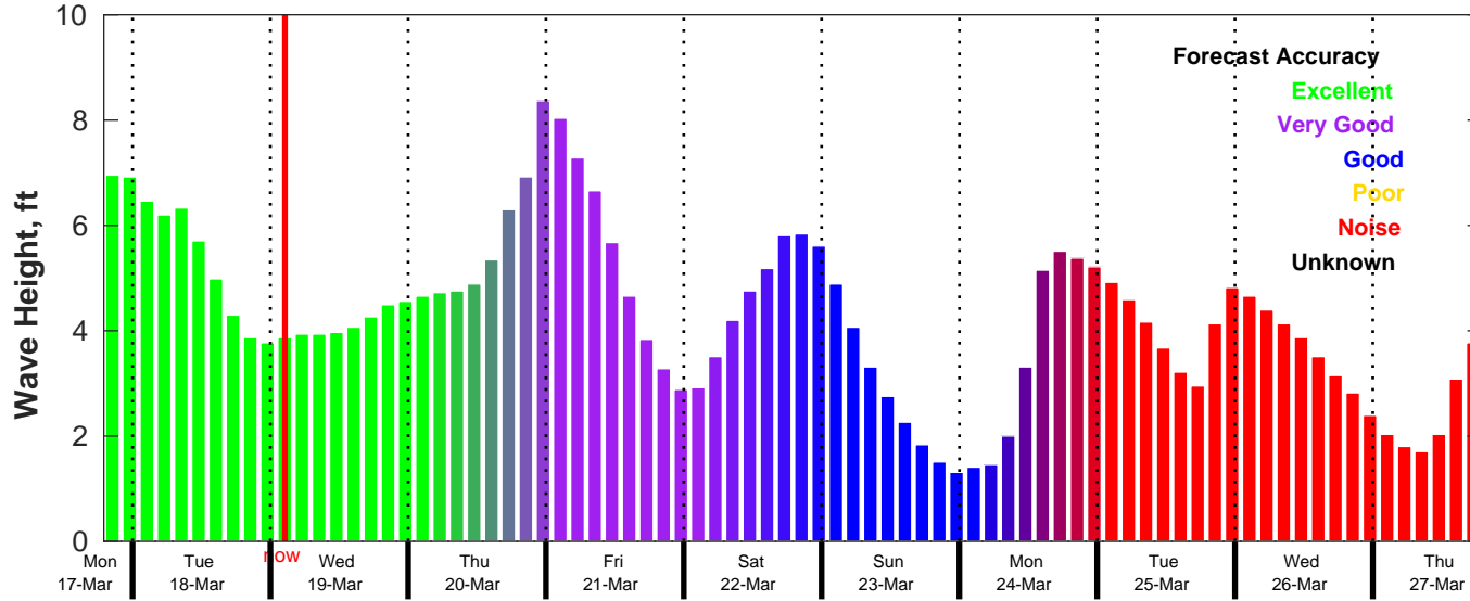
CMEMS Wave Forecast for NDBC 41013 from 17-Mar-2025 19:00:00 to 27-Mar-2025 19:00:00
