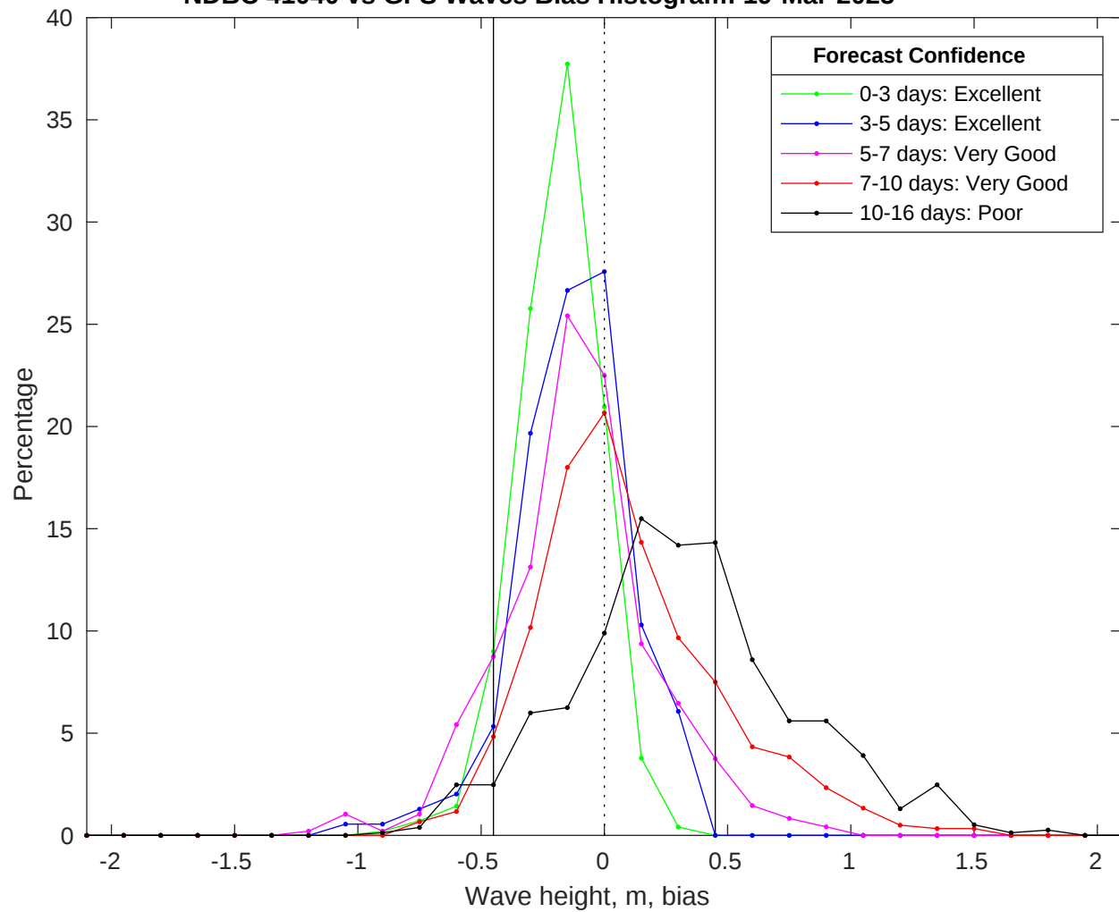
NDBC 41040 vs GFS Waves Bias Histogram: 19-Mar-2025
