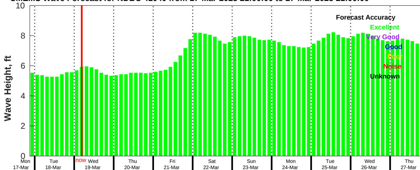
CMEMS Wave Forecast for NDBC 41040 from 17-Mar-2025 21:00:00 to 27-Mar-2025 21:00:00
