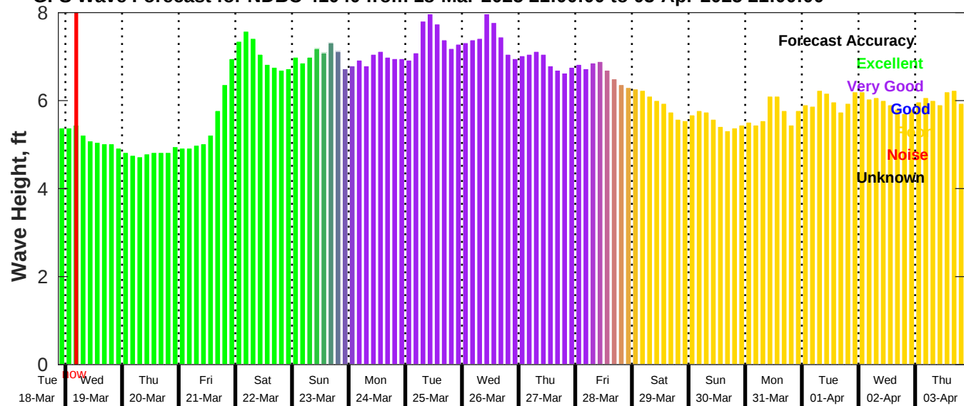
GFS Wave Forecast for NDBC 41040 from 18-Mar-2025 21:00:00 to 03-Apr-2025 21:00:00
