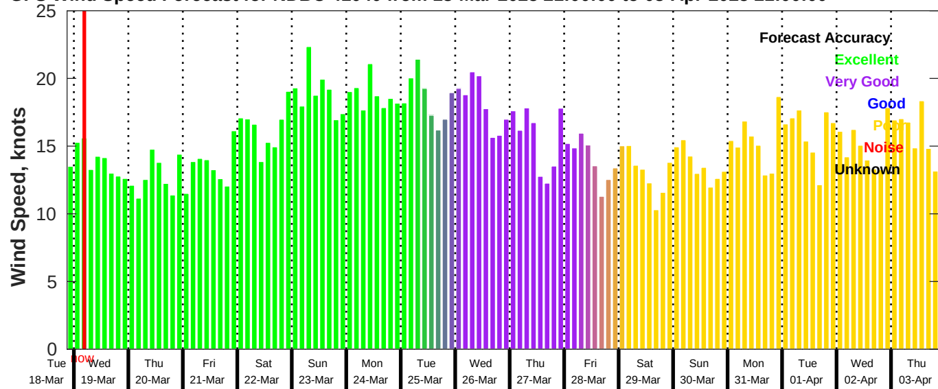
GFS Wind Speed Forecast for NDBC 41040 from 18-Mar-2025 21:00:00 to 03-Apr-2025 21:00:00
