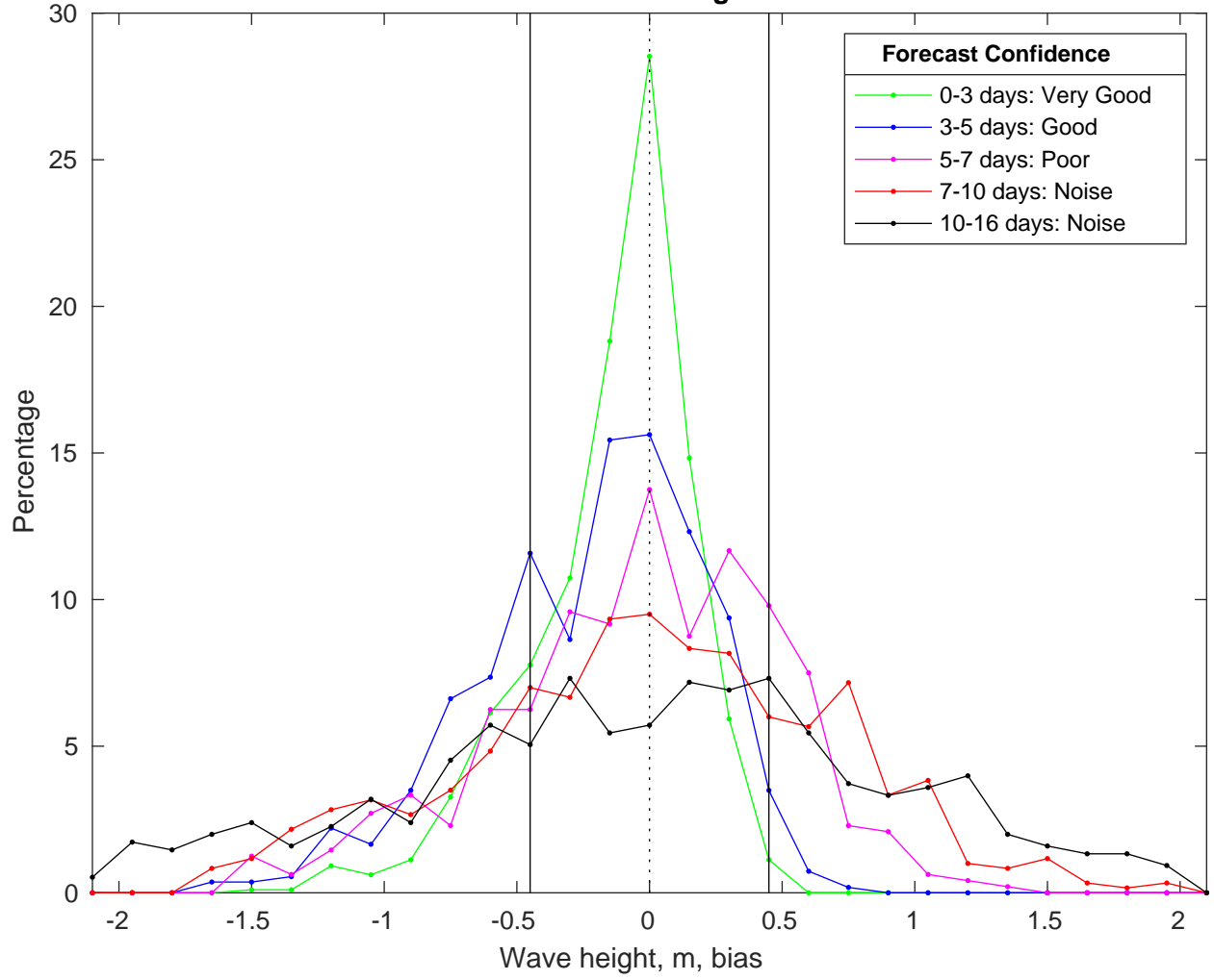
NDBC 42019 vs GFS Waves Bias Histogram: 19-Mar-2025
