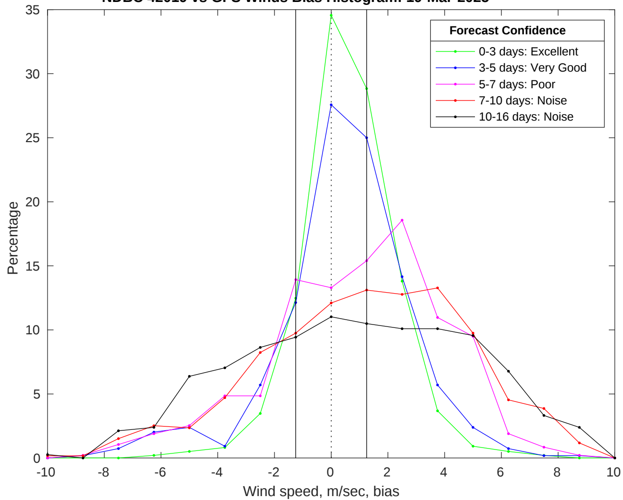
NDBC 42019 vs GFS Winds Bias Histogram: 19-Mar-2025
