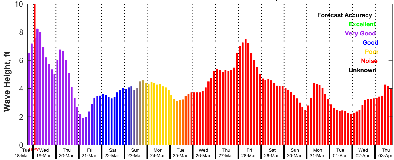
GFS Wave Forecast for NDBC 42019 from 18-Mar-2025 18:00:00 to 03-Apr-2025 18:00:00
