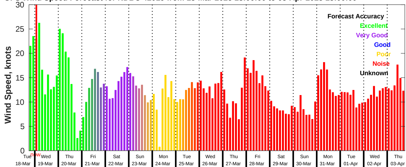
GFS Wind Speed Forecast for NDBC 42019 from 18-Mar-2025 18:00:00 to 03-Apr-2025 18:00:00
