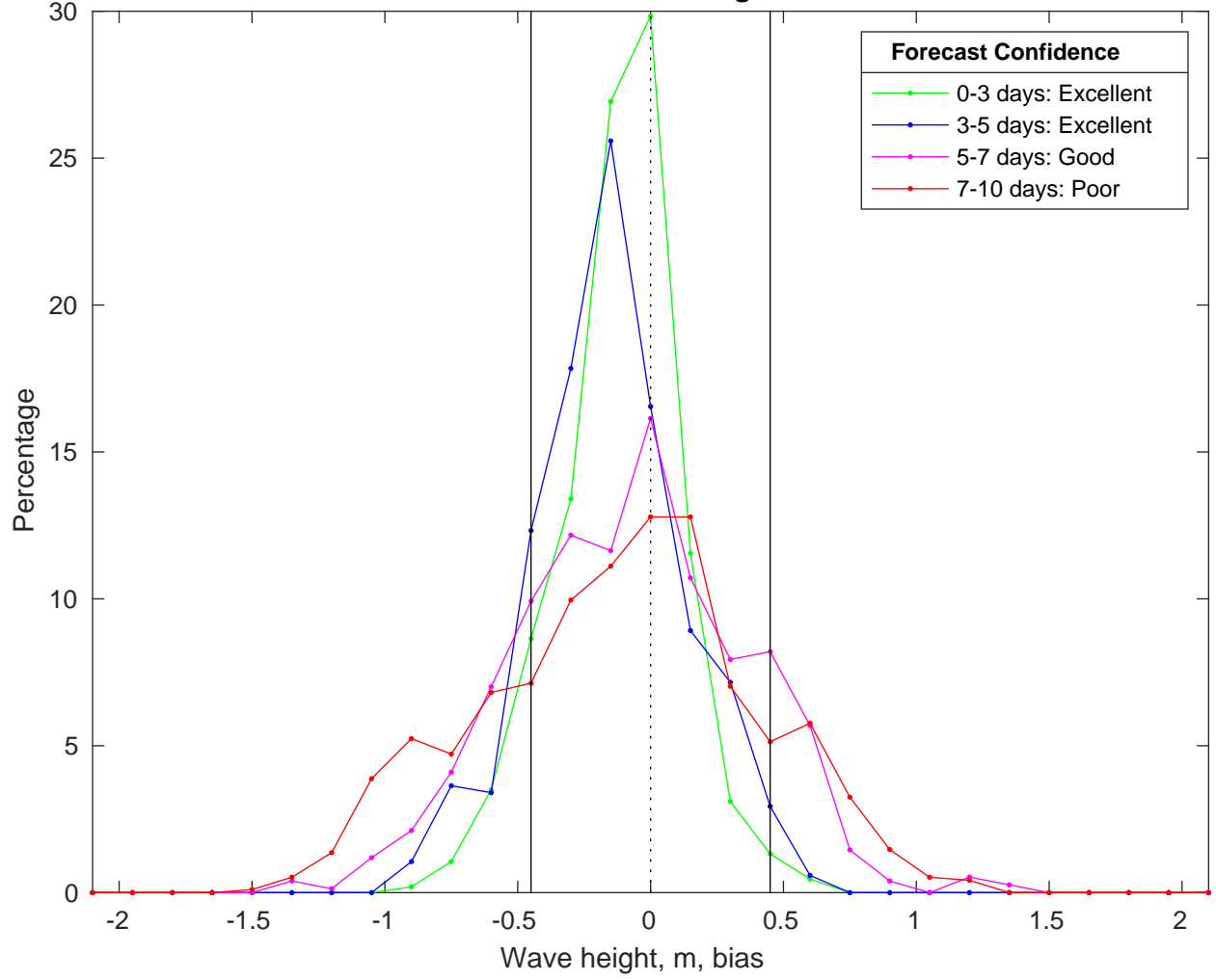
NDBC 42020 vs CMEMS Waves Bias Histogram: 19-Mar-2025
