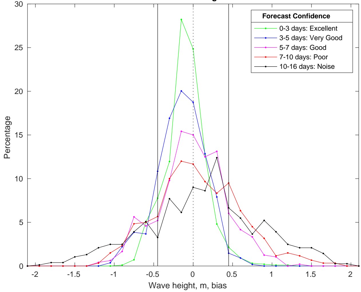
NDBC 42020 vs GFS Waves Bias Histogram: 19-Mar-2025
