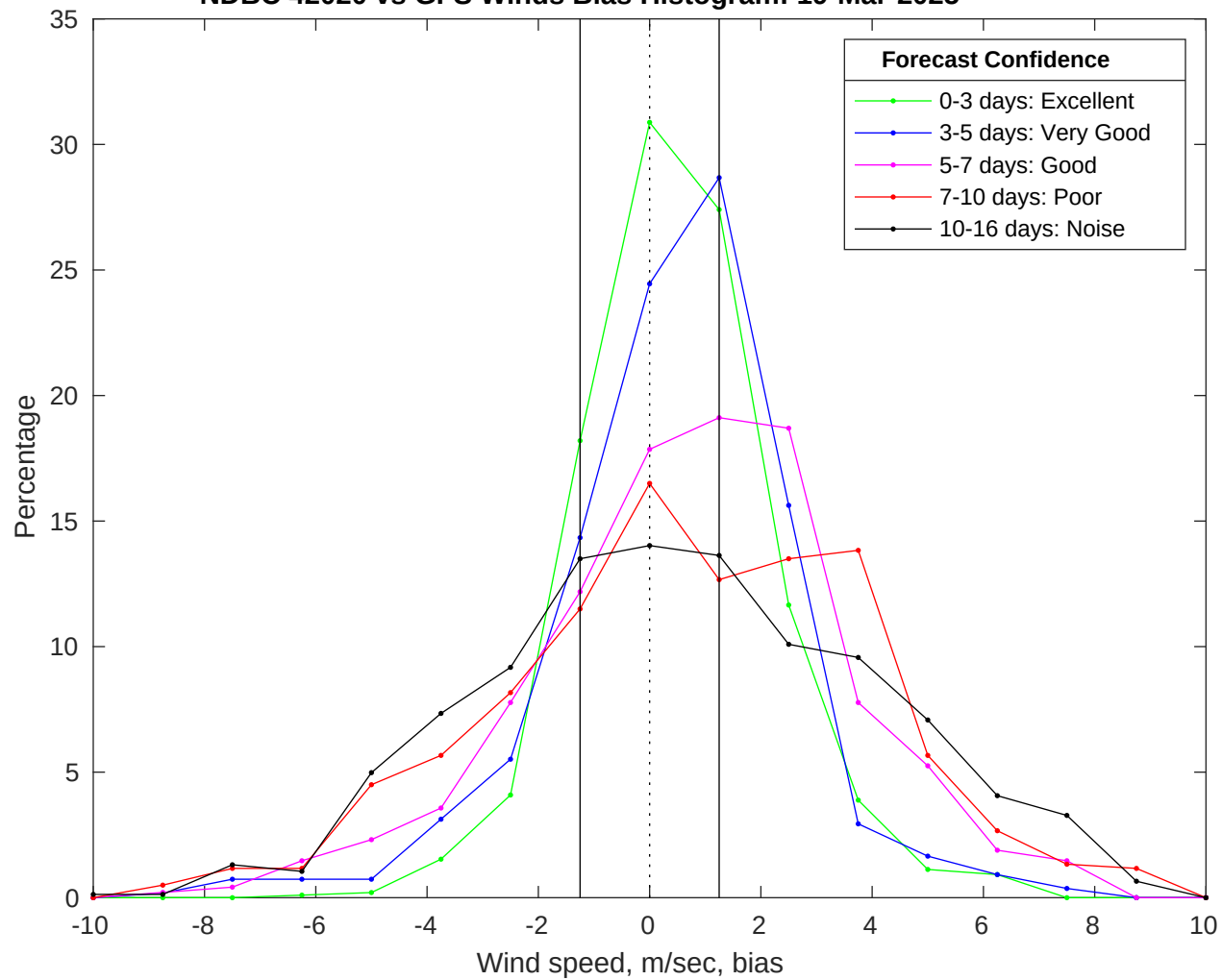
NDBC 42020 vs GFS Winds Bias Histogram: 19-Mar-2025
