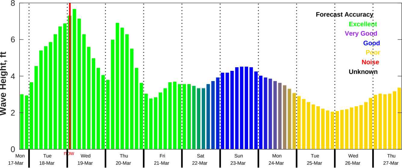
CMEMS Wave Forecast for NDBC 42020 from 17-Mar-2025 18:00:00 to 27-Mar-2025 18:00:00
