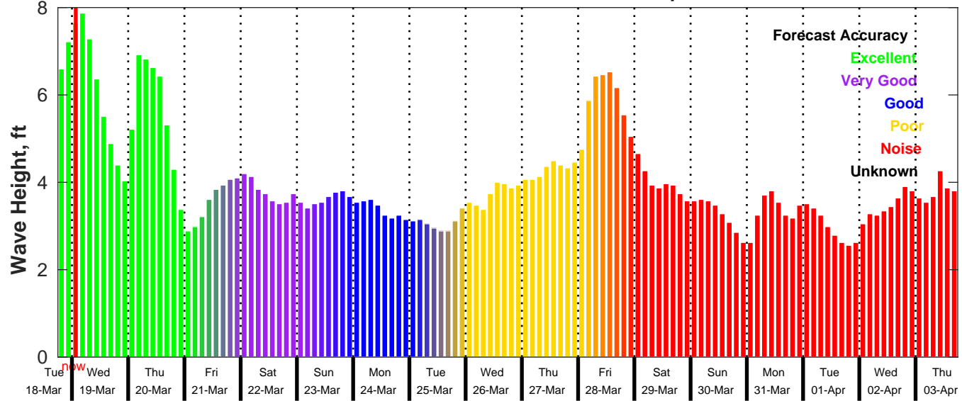
GFS Wave Forecast for NDBC 42020 from 18-Mar-2025 18:00:00 to 03-Apr-2025 18:00:00
